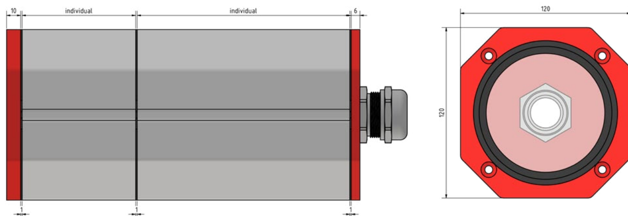
Standard dimensions of the CH87 housing with M32 cable gland, IP69 (mm).
